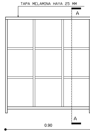
VISTA FRONTAL
