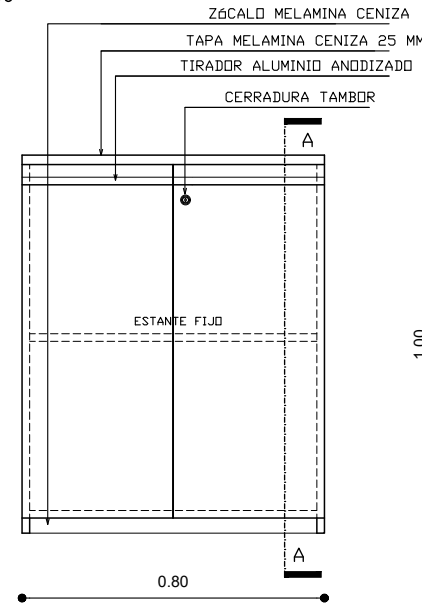
VISTA FRONTAL
