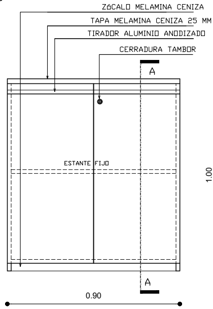
VISTA FRONTAL
