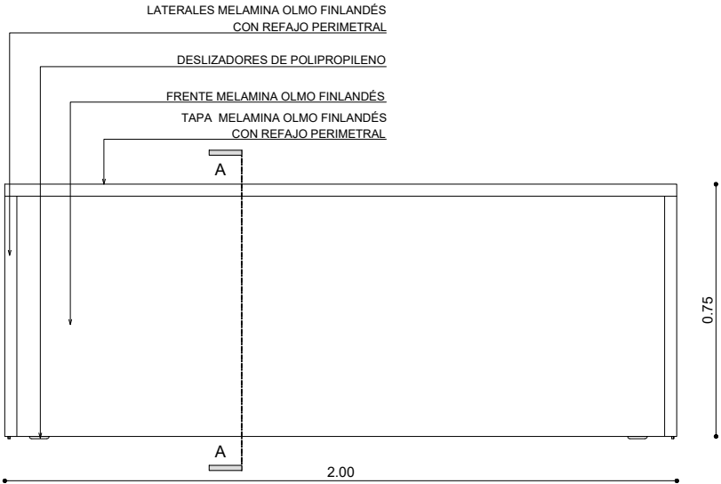
VISTA FRONTAL
